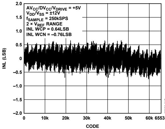
Figure 6. AD7656 Typical INL
